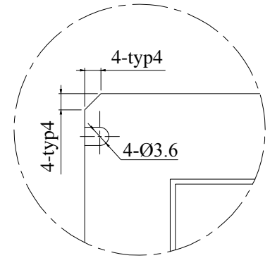
Detail B 3:1
