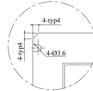
Detail B 3:1
