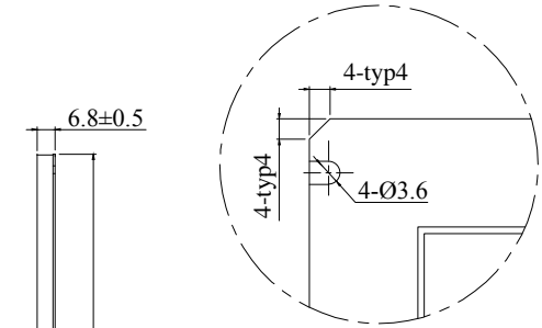
Detail B 3:1
