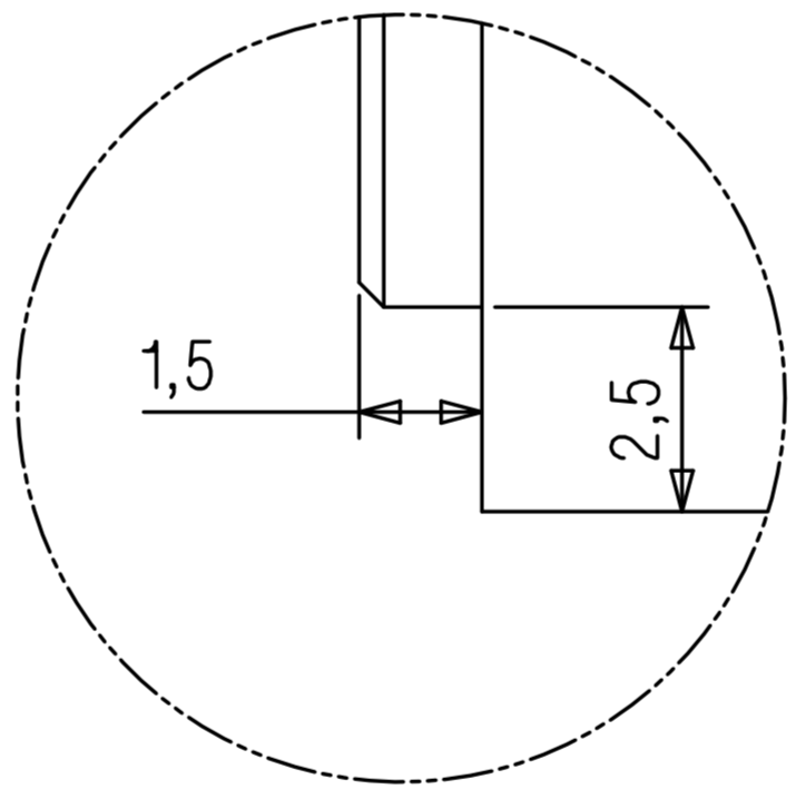
DETAIL M SCALE 10/1
