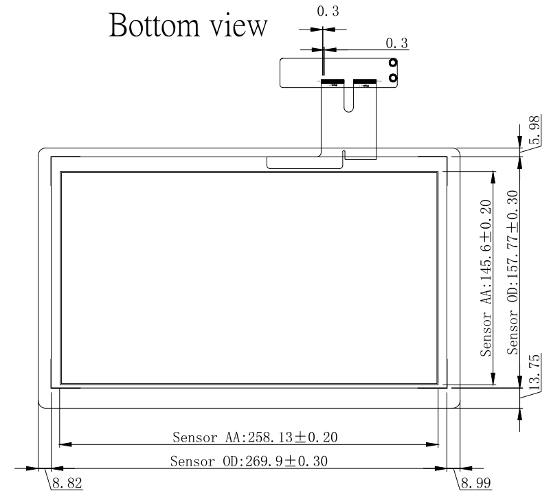
Touch Panel Structure
