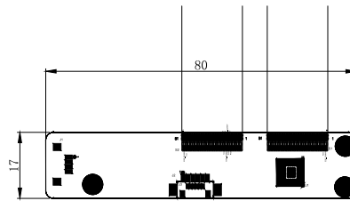
Detail A (3:1)
